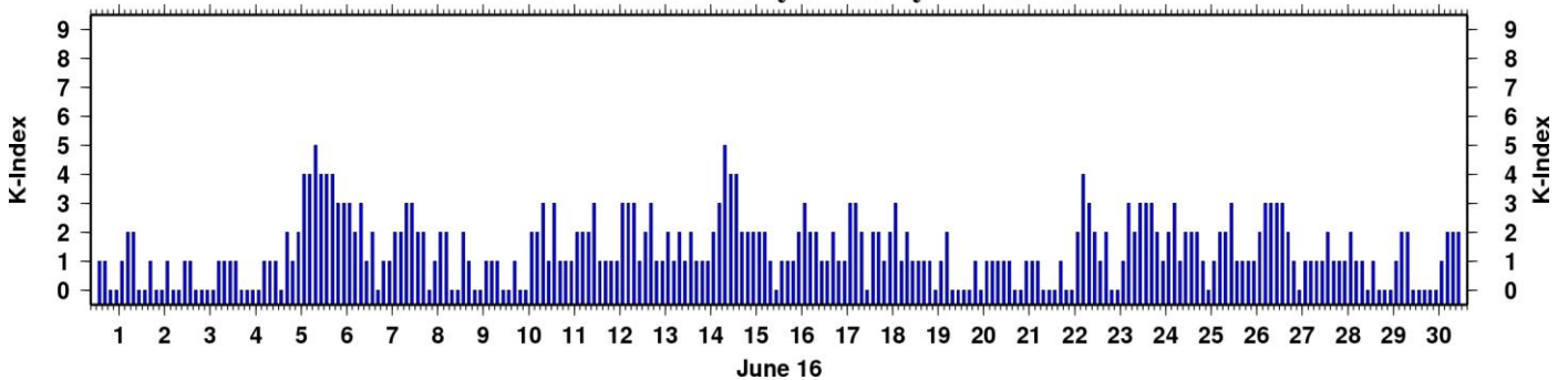
Lerwick Observatory 3-hourly K-Indices
