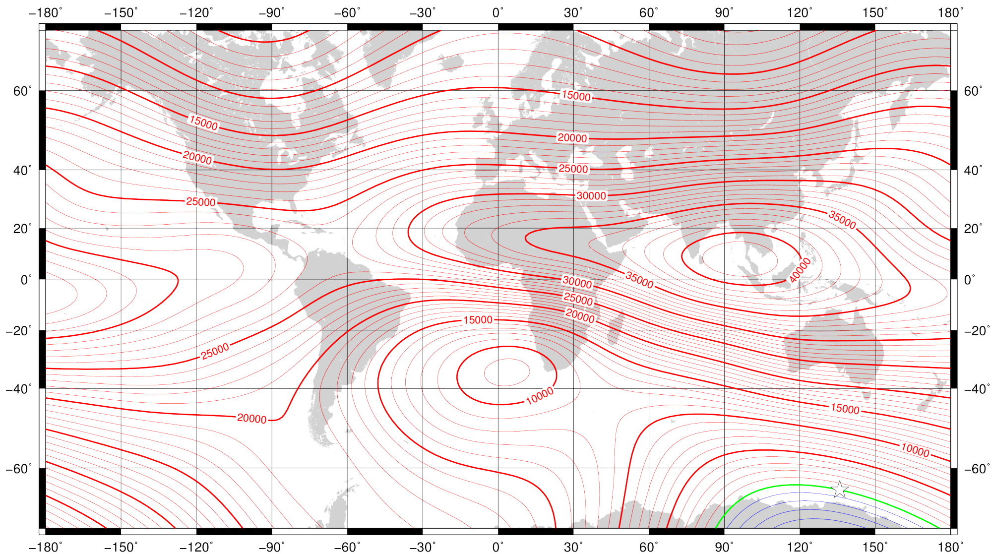
North component ( X ) at 2020.0 from the World Magnetic Model (WMM2020). Red – positive (north), blue – negative (south), green – zero. Contour interval is 1000 nT, white star is location of a magnetic pole and projection is Mercator. This is an example of an isodynamic chart. Credit: British Geological Survey (UK Research and Innovation).
