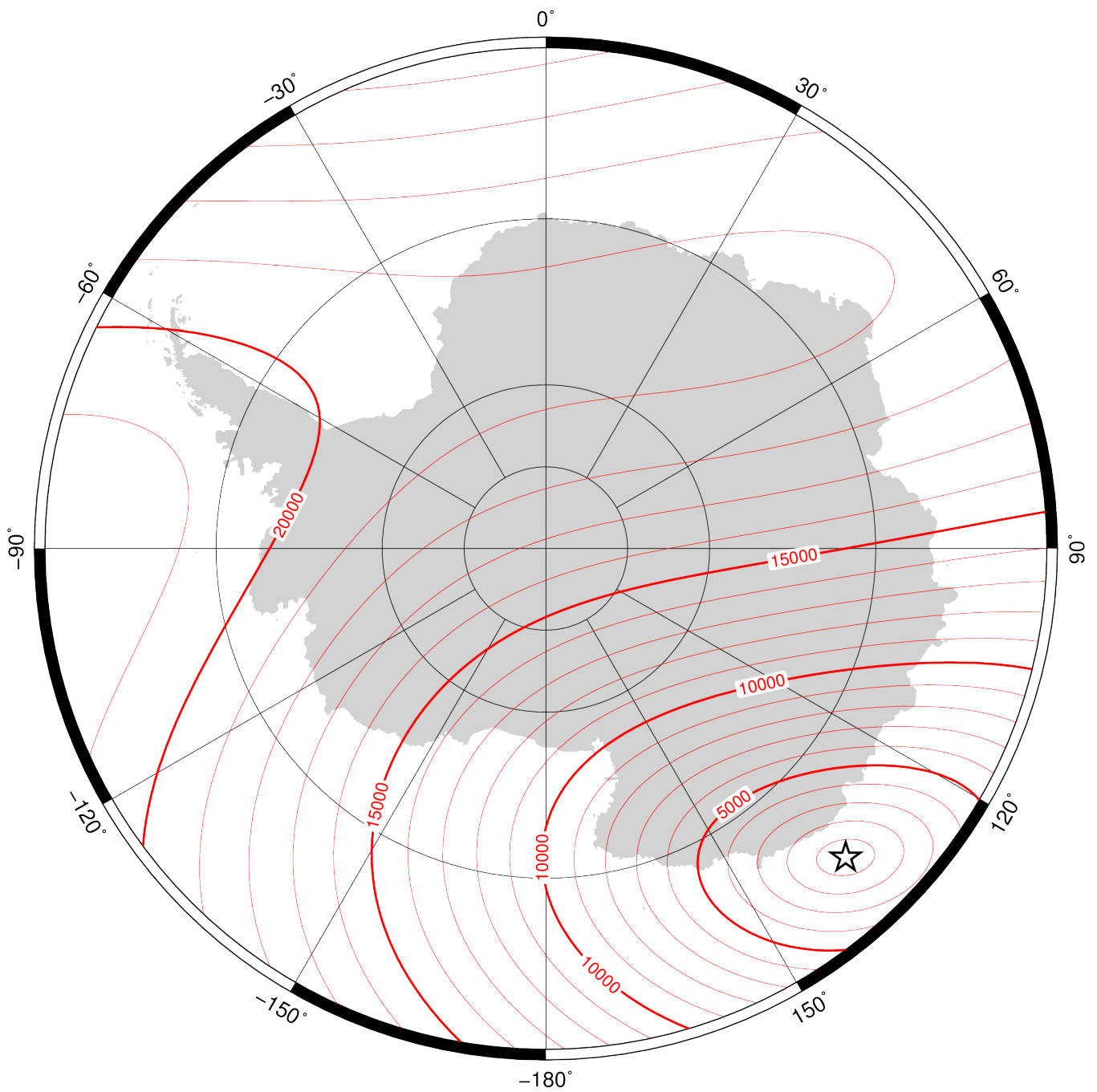
Horizontal intensity ( H ) in region of south pole at 2020.0 from the World Magnetic Model (WMM2020). Contour interval is 1000 nT, white star is location of a magnetic pole and projection is Polar Stereographic. Credit: British Geological Survey (UK Research and Innovation).
